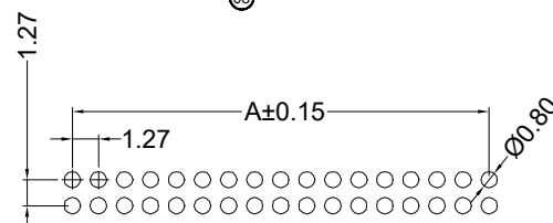
P.C.B Board Layout
