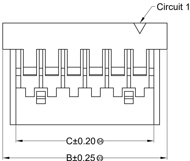
03P~30P Double Salient
